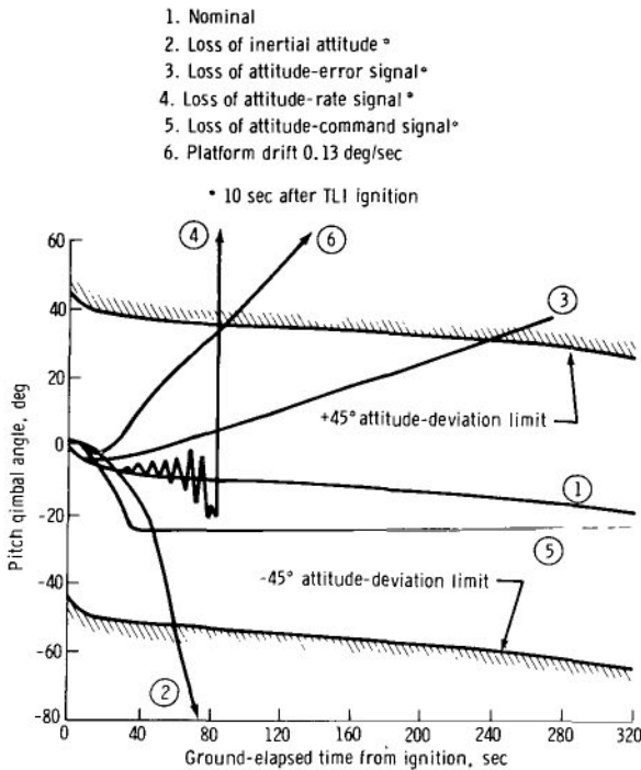
Figure 9. - Malfunctions during TLI.
