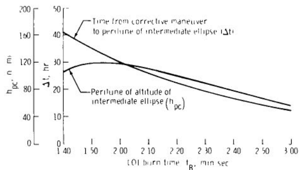
Figure 21. - Time between burns and the pericynthion altitude following a nominal first burn for an LOI mode II abort.
