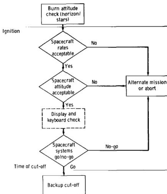
Figure 8. - Basic crew-maneuver-monitoring technique.
