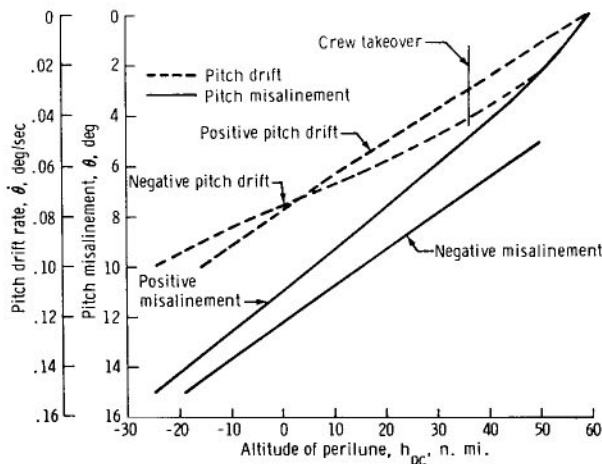
Figure 14. - Effects of attitude-reference failures on pericynthion altitude.
