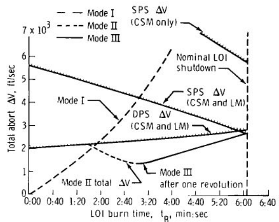
Figure 19. - Summary of minimum-fuel abort capability as a function of LOI burn time.
